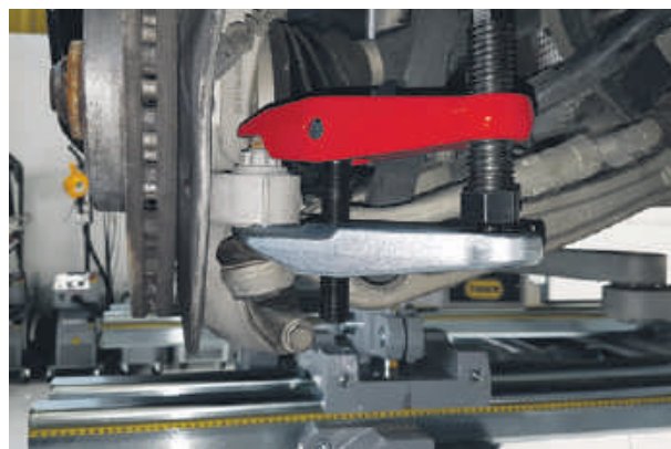
Audi - demontage spoorstangkop
